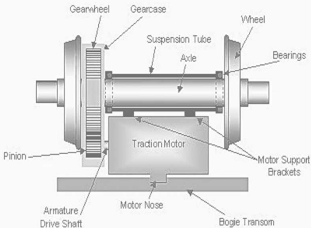
Diagram of DC Nose Suspended Traction Motor
